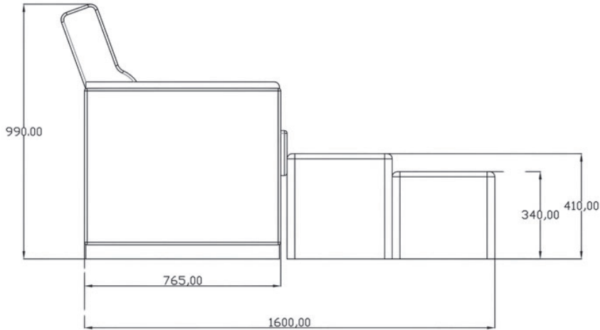
MAXIMUM HEIGHT
