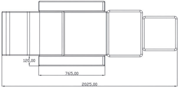
TOP VIEW (IN RECLINE BACKREST POSITION)
