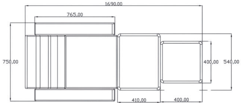
TOP VIEW (IN INCLINE BACKREST POSITION)
