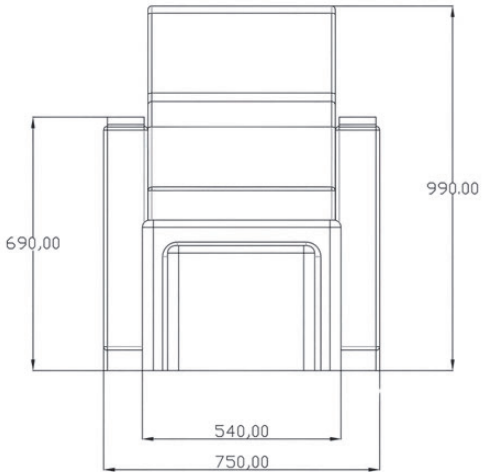
TOP VIEW (IN CHAIR POSITION)
