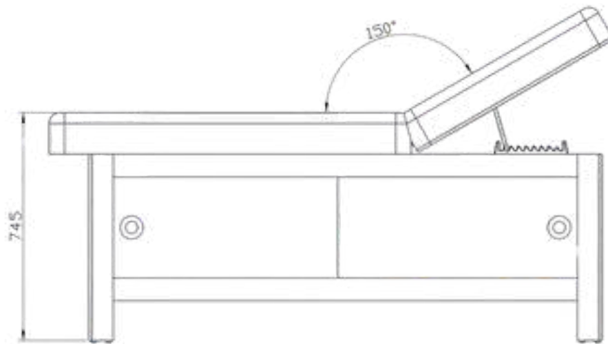
SIDE VIEW
